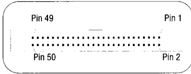
Figure 3 Internal Connector
