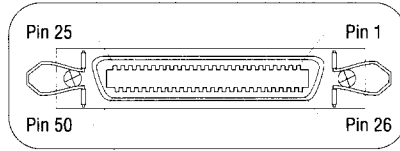
Figure 4 Device Connector
